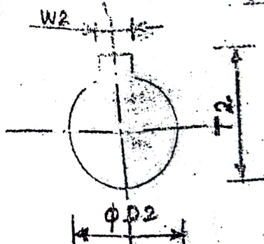
DRIVEN SIDE BORE DETAIL MACHINE SIDE
